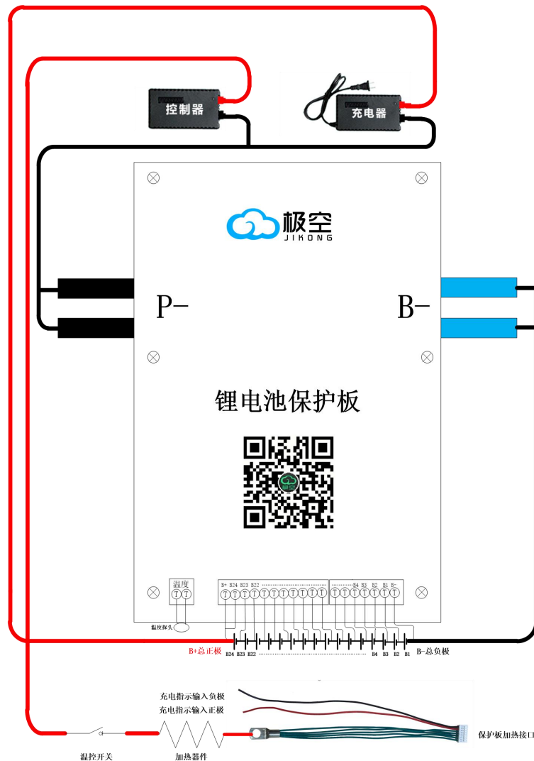
JK-BxAxxS-15P/20P-24S接线图
