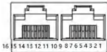
RS485A
