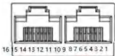
RS485
